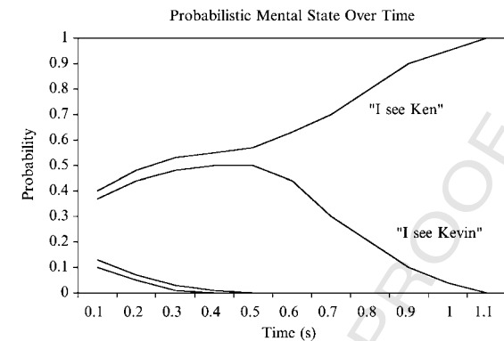
Fig. 4. An idealized evolution of these probabilistic activations (or normalized proximities) depicting a dynamic graded mental state over the course of several hundred milliseconds.
