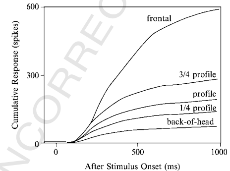
Fig. 16. The accumulation over time of neuronal spikes (over and above the baseline spike rate) from cells responding to faces at various rotations around the vertical axis (adapted from Perrett et al., 1998).
