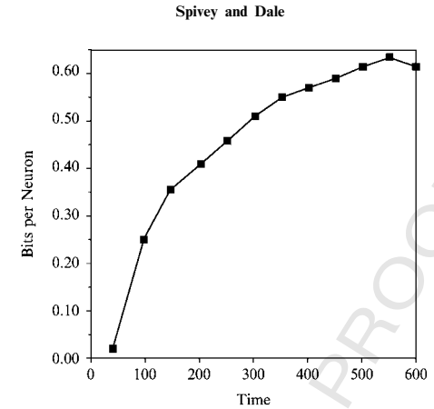
Fig. 15. Average cumulative information accrued over milliseconds by inferotemporal cells representing objects and faces (adapted from Rolls & Tovee, 1995).
