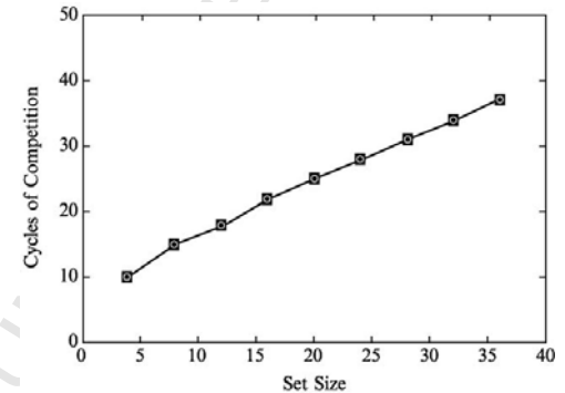
Fig. 18. Settling times for normalized recurrence during a conjunction search with different set sizes.
