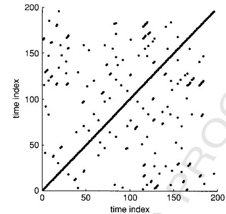
Fig. 23. In this very simple example of a recurrence plot, a series of sine values with some noise added was subjected to embedding. The diagonal is the line of identity, where i = j , and one can observe further diagonal structure emerging at other time indices, indicating some periodicity in the noisy sinusoidal time series.
