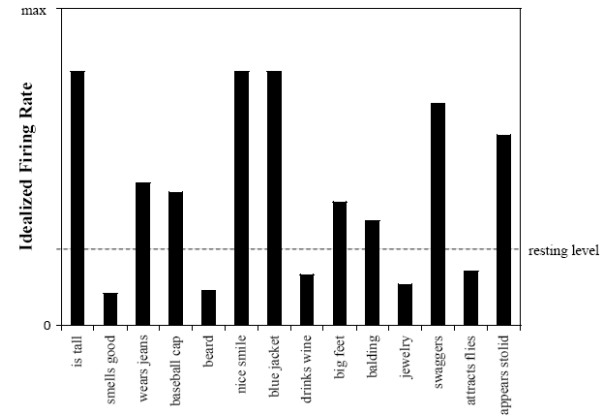
Fig. 2. Idealized labels for each neuron in the graded brain state.
