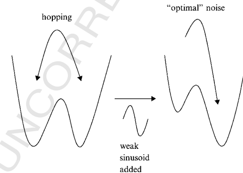
Fig. 21. When a weak sinusoid is added to an equibased stochastic process, resonance can produce a significantly biased stochastic process.
