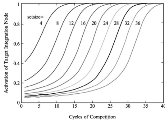
Fig. 19. In normalized recurrence, the winning node's activation rises with a sigmoid function, but this curve shifts linearly in time as set size increases.
